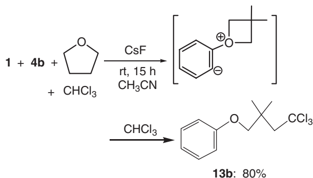
Scheme 10.
