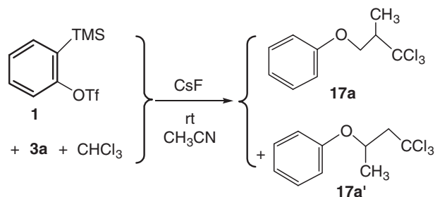
Scheme 12.
