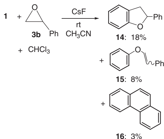
Scheme 11.
