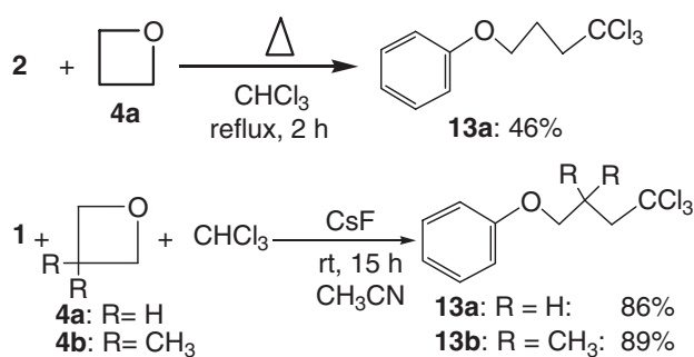
Scheme 9.
