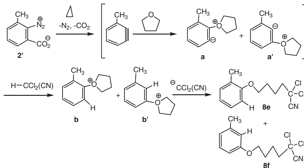
Scheme 6.
